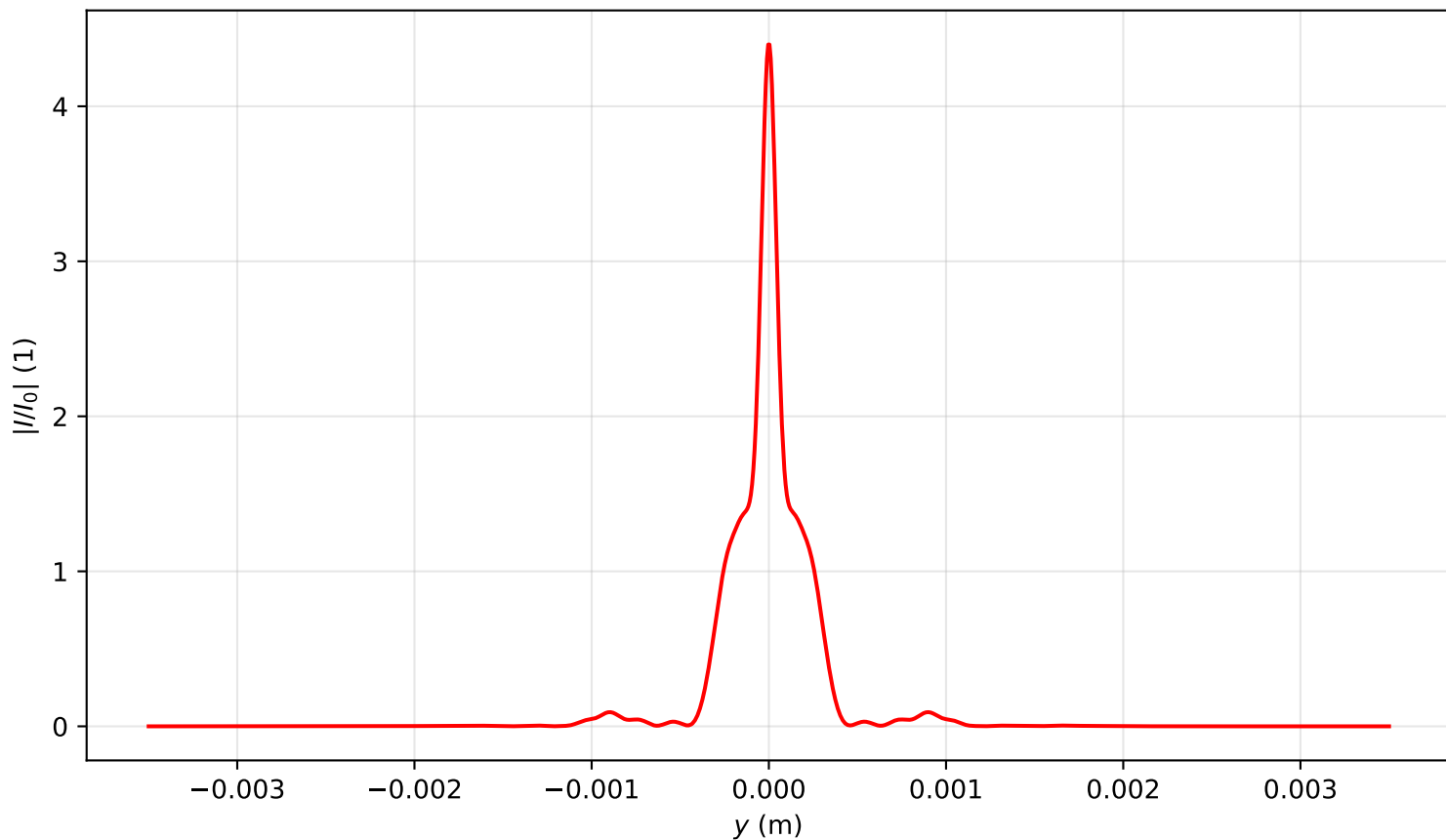
Intensity profile I(x=0, y, z=1.194)/I_0 , \text{Pin}=5.0\text{Pcr} , artificial time
